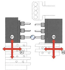
Opposing simultaneous cross drilling
