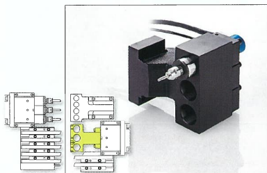
Triple holder for high-speed drilling unit
