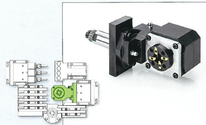
Thread whirling unit
