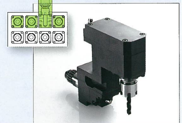
Cross drilling unit (for back working)
