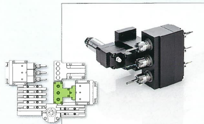
3-spindle opposing type front drilling unit
