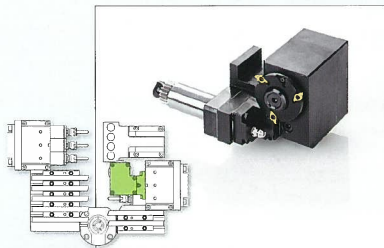
Polygon machining unit
