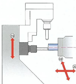
Back off-center face drilling/milling
