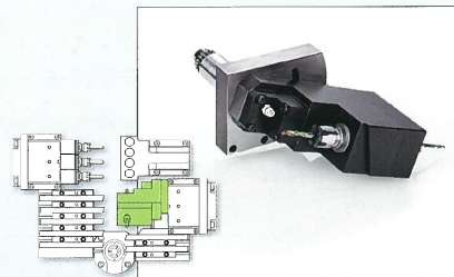
Angular hole drilling unit adjustable type
