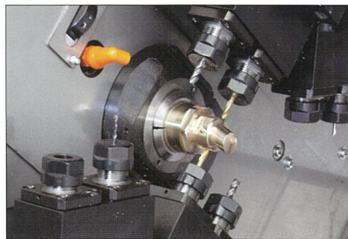
Cross Drilling + Cross Milling
