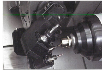
Skewed Hole Drilling
