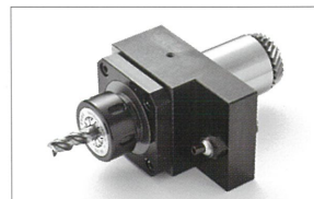
Milling unit ER25
