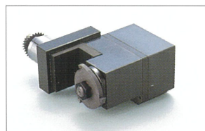
Polygon machining unit
