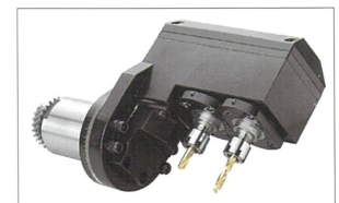
2-spindle skewed hole drilling unit
