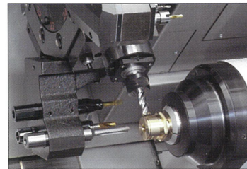
Back Cross Milling
